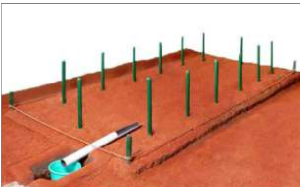
FIXING OF PEGS
